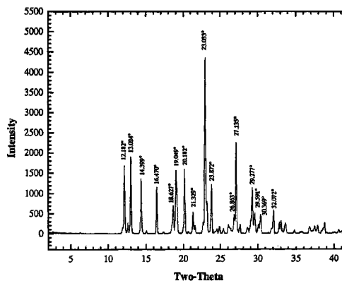
X-ray Powder Diffraction Pattern of Azacytidine, Form I, Labeled with the more Prominent 2 \theta Angles (Cu K \alpha Radiation)
